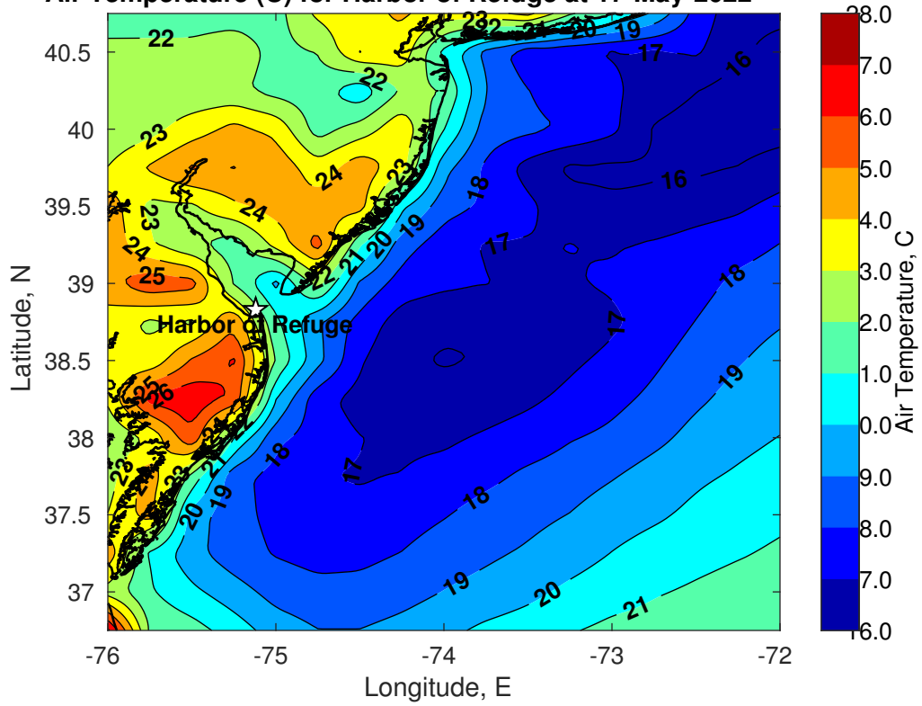
Air Temperature (C) for Harbor of Refuge at 17-May-2022
