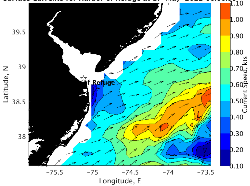
Surface Currents for Harbor of Refuge at 17-May-2022 00:00:00
