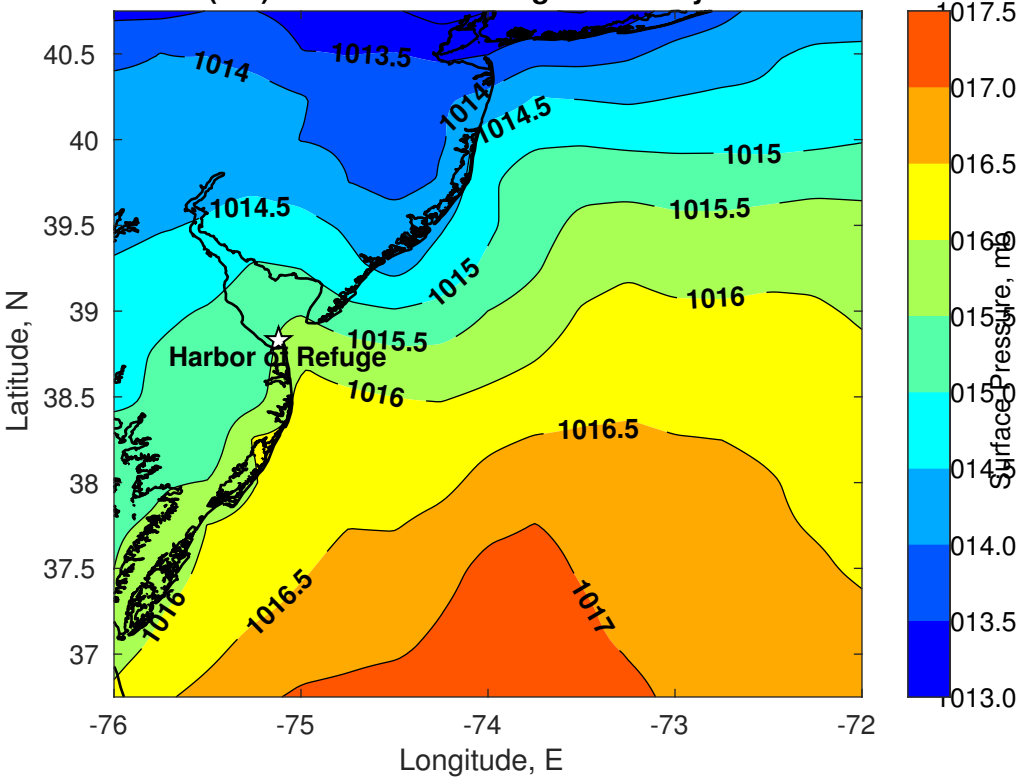
Surface Pressure (mb) for Harbor of Refuge at 18-May-2022 21:00:00
