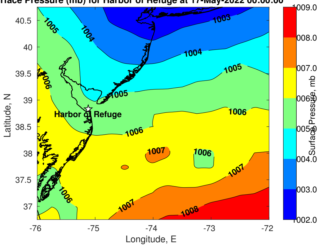
Surface Pressure (mb) for Harbor of Refuge at 17-May-2022 00:00:00
