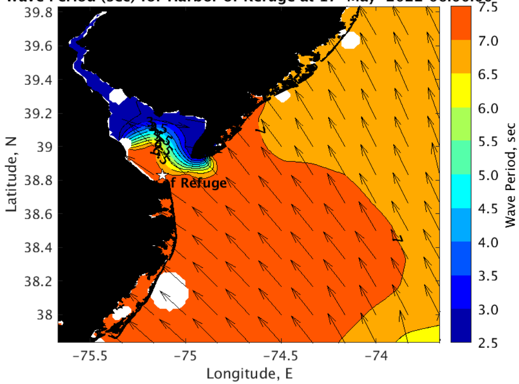
Wave Period (sec) for Harbor of Refuge at 17-May-2022 06:00:00
