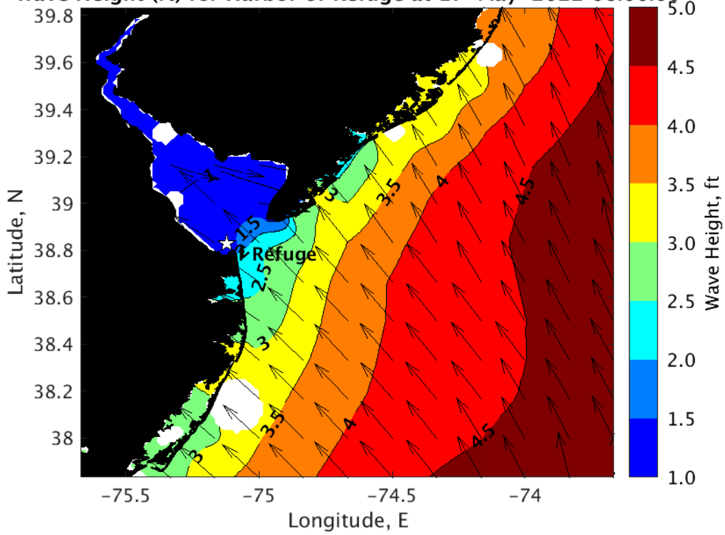
Wave Height (ft) for Harbor of Refuge at 17-May-2022 06:00:00
