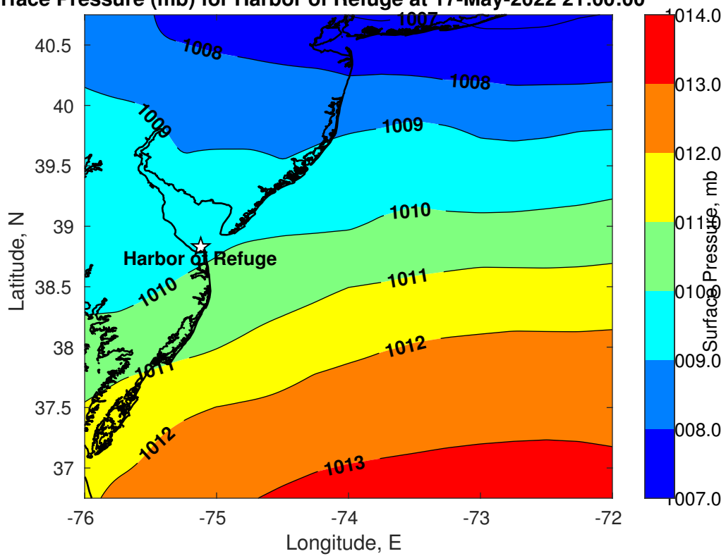
Surface Pressure (mb) for Harbor of Refuge at 17-May-2022 21:00:00
